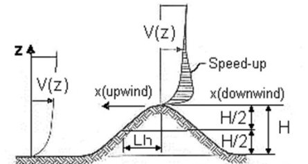
2D RIDGE or 3D AXISYMMETRICAL HILL
